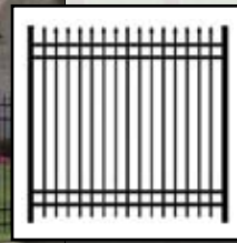
Model 0141 - 4 Rail - with Spears Height: 72" • Length: 6' Sections
